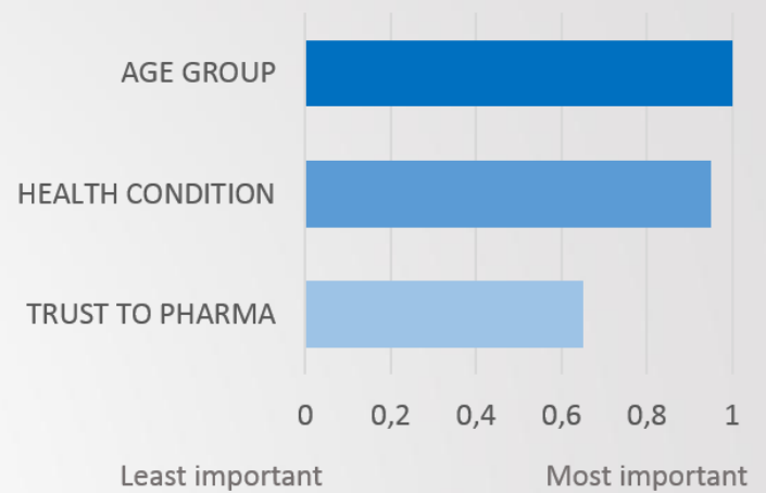
Predictor Importance
