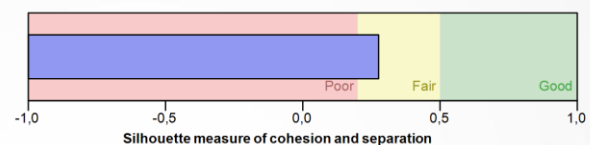
Cluster Quality
